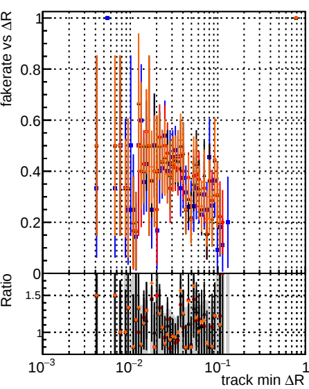
Fake rate vs \Delta R(\text{track, jet}) DOM original_step2_ttbar-phase1-newgeom DOM pixelCPE_template_step2_ttbar-phase1-newgeom DOM pixelCPE_template_cutChiSquareNew2_step2_ttbar-phase1-newgeom DOM pixelCPE_template_cutChiSquareNew2_step2_ttbar-phase1-newgeom
