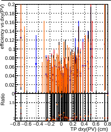
Efficiency vs Dxy(PV) DQM_original_step2_ttbar-phase1-newgeom DQM_pixelCPETemplate_step2_ttbar-phase1-newgeom DQM_pixelCPETemplateCutChiSquare15_step2_ttbar-phase1-newgeom DQM_pixelCPETemplateCutChiSquare5_step2_ttbar-phase1-newgeom_test
