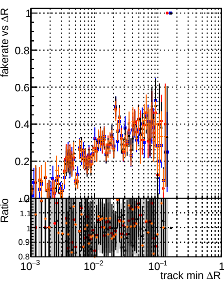
Fake rate vs \Delta R(\text{track, jet}) DOM original_step2_ttbar-phase1-newgeom DOM pixelCPE Etemplate_step2_ttbar-phase1-newgeom DOM pixelCPE Etemplate_CurChisquare5_step2_ttbar-phase1-newgeom DOM pixelCPE Etemplate_CurChisquare5_step2_ttbar-phase1-newgeom_test
