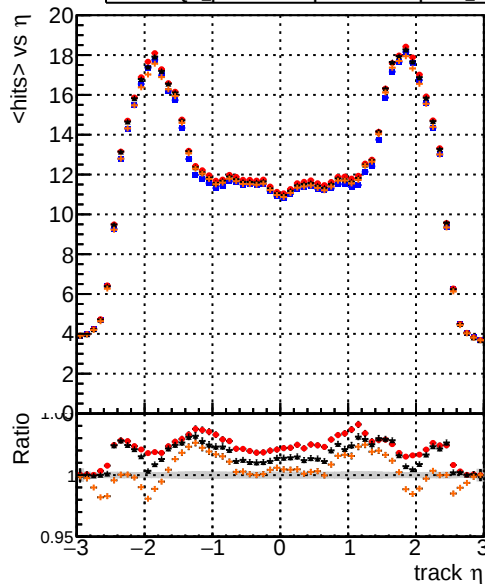
mean hits — DQM_original_step2_ttbbar-phase1-newgeom — DQM_pixelCPETemplate_step2_ttbbar-phase1-newgeom — DQM_pixelCPETemplateCutChiSquare15_step2_ttbbar-phase1-newgeom — DQM_pixelCPETemplateCutChiSquare5_step2_ttbbar-phase1-newgeom_test
