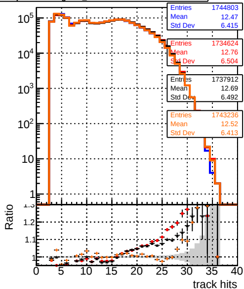
mean hits — DQM_original_step2_ttbbar-phase1-newgeom — DQM_pixelCPETemplate_step2_ttbbar-phase1-newgeom — DQM_pixelCPETemplateCutChiSquare15_step2_ttbbar-phase1-newgeom — DQM_pixelCPETemplateCutChiSquare5_step2_ttbbar-phase1-newgeom_test
