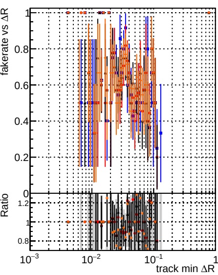
Fake rate vs \Delta R(\text{track, jet}) DOM original_step2_ttbar-phase1-newgeom DOM pixelCPE-template_step2_ttbar-phase1-newgeom DOM pixelCPE-template_ChiSquare5_step2_ttbar-phase1-newgeom DOM pixelCPE-template_ChiSquare5_step2_ttbar-phase1-newgeom_test
