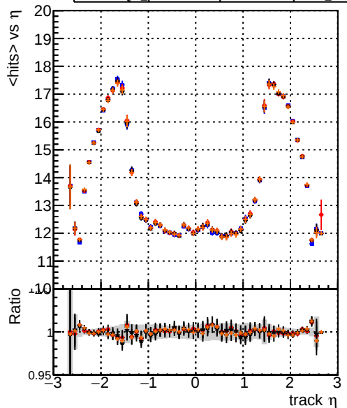
mean hits vs \eta — DQM_original_step2_ttbar-phase1-newgeom — DQM_pixelCPETemplate_step2_ttbar-phase1-newgeom — DQM_pixelCPETemplateCutChiSquare15_step2_ttbar-phase1-newgeom — DQM_pixelCPETemplateCutChiSquare5_step2_ttbar-phase1-newgeom_test
