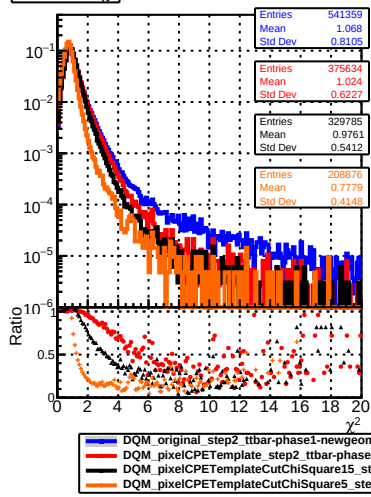
normalized \chi^2
