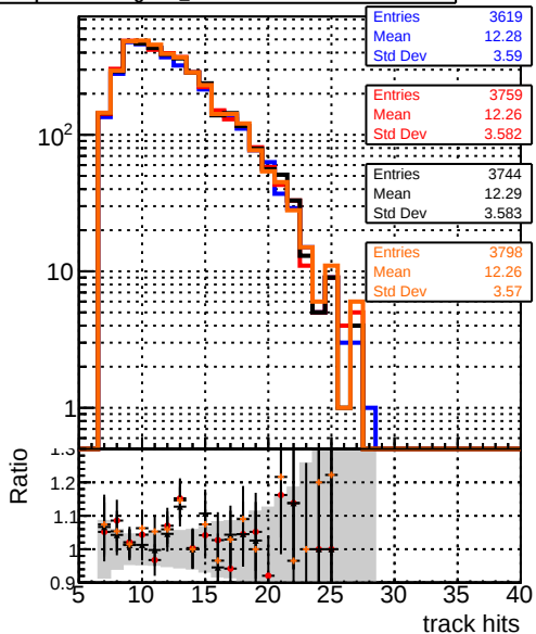
mean hits DQM_original_step2_ttbbar-phase1-newgeom DQM_pixelCPETemplate_step2_ttbbar-phase1-newgeom DQM_pixelCPETemplateCutChiSquare15_step2_ttbbar-phase1-newgeom DQM_pixelCPETemplateCutChiSquare5_step2_ttbbar-phase1-newgeom_test
