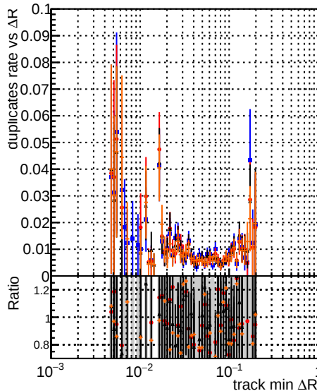
DOM original, step2, ttbar, phase1, newgeom pixelCPE, template, cut, chiSquare, test DOM original, step2, ttbar, phase1, newgeom pixelCPE, template, cut, chiSquare, test
