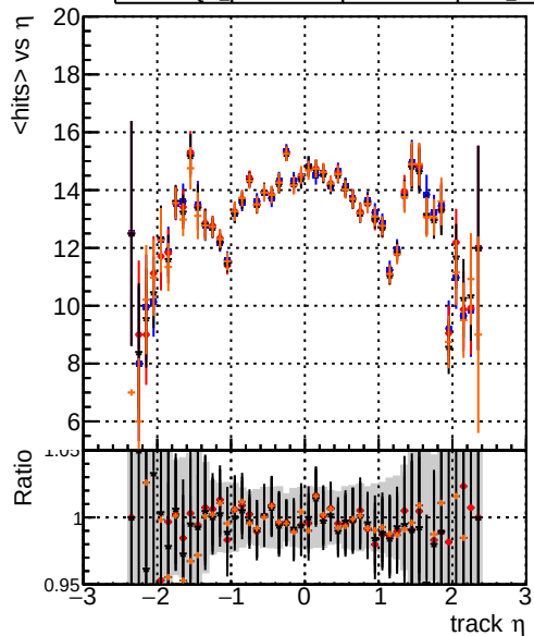
mean hits — DQM_originalStep2_ttbar-phase1-newgeom — DQM_pixelCPETemplate_step2_ttbar-phase1-newgeom — DQM_pixelCPETemplateCutChiSquare15_step2_ttbar-phase1-newgeom — DQM_pixelCPETemplateCutChiSquare5_step2_ttbar-phase1-newgeom_test
