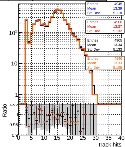
mean hits — DQM_originalStep2_ttbar-phase1-newgeom — DQM_pixelCPETemplate_step2_ttbar-phase1-newgeom — DQM_pixelCPETemplateCutChiSquare15_step2_ttbar-phase1-newgeom — DQM_pixelCPETemplateCutChiSquare5_step2_ttbar-phase1-newgeom_test
