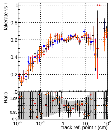
DOM original step2 ttbar-phase1-newgeom DOM pixel CDF template step2 ttbar-phase1-newgeom DOM pixel CDF template ChiSquare step2 ttbar-phase1-newgeom DOM pixel CDF template ChiSquare step2 ttbar-phase1-newgeom test
