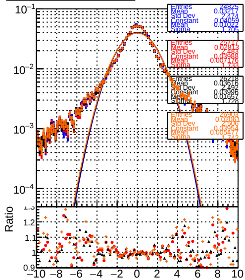
pull of q_{\text{over}} \text{ parameter}
