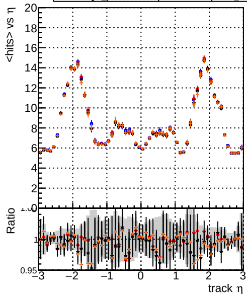
mean hits — DQM_original_step2_ttbar-phase1-newgeom — DQM_pixelCPETemplate_step2_ttbar-phase1-newgeom — DQM_pixelCPETemplateCutChiSquare15_step2_ttbar-phase1-newgeom — DQM_pixelCPETemplateCutChiSquare5_step2_ttbar-phase1-newgeom_test
