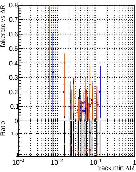
Fake rate vs \Delta R(\text{track, jet}) Legend: DOM original (blue) DOM pixel (red) DOM template (black) DOM chi-square (orange) DOM original step2 (blue) DOM pixel step2 (red) DOM template step2 (black) DOM chi-square step2 (orange) DOM original phase1 (blue) DOM pixel phase1 (red) DOM template phase1 (black) DOM chi-square phase1 (orange) DOM original newgeom (blue) DOM pixel newgeom (red) DOM template newgeom (black) DOM chi-square newgeom (orange) DOM original test (blue) DOM pixel test (red) DOM template test (black) DOM chi-square test (orange)
