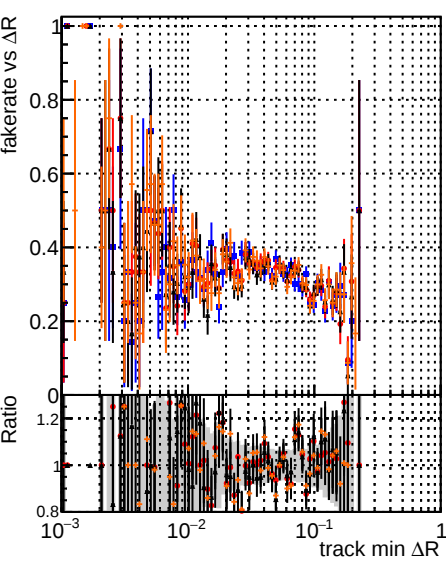
Fake rate vs \Delta R(\text{track, jet}) Legend: DOM original, step2, ttbar, phase1, newgeom pixelCPE, template, cutchisquare5, step2, ttbar, phase1, newgeom DOM original, step2, ttbar, phase1, newgeom pixelCPE, template, cutchisquare5, step2, ttbar, phase1, newgeom DOM original, step2, ttbar, phase1, newgeom pixelCPE, template, cutchisquare5, step2, ttbar, phase1, newgeom
