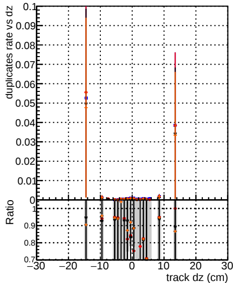
Square15_step2 ttbar-phase1-newgeom
