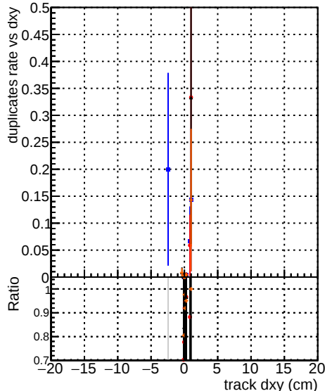
Square15_step2 ttbar-phase1-newgeom
