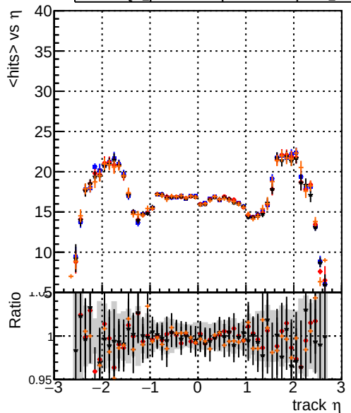
mean hits — DQM_original step2 ttbar-phase1-newgeom — DQM_pixelCPETemplate_step2 ttbar-phase1-newgeom — DQM_pixelCPETemplateCutChiSquare15_step2 ttbar-phase1-newgeom — DQM_pixelCPETemplateCutChiSquare5_step2 ttbar-phase1-newgeom_test
