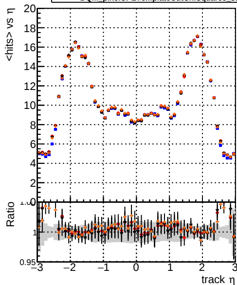
mean hit — DQM_original_step2_ttbbar-phase1-newgeom — DQM_pixelCPETemplate_step2_ttbbar-phase1-newgeom — DQM_pixelCPETemplateCutChiSquare15_step2_ttbbar-phase1-newgeom — DQM_pixelCPETemplateCutChiSquare5_step2_ttbbar-phase1-newgeom_test
