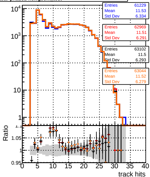
mean hit — DQM_original_step2_ttbbar-phase1-newgeom — DQM_pixelCPETemplate_step2_ttbbar-phase1-newgeom — DQM_pixelCPETemplateCutChiSquare15_step2_ttbbar-phase1-newgeom — DQM_pixelCPETemplateCutChiSquare5_step2_ttbbar-phase1-newgeom_test
