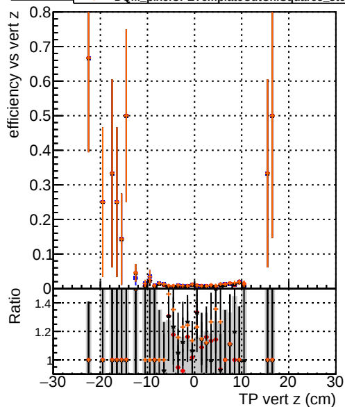
Efficiency DOM_pixelCPETemplateCutChiSquare155_step2 ttbar-phase1-newgeom DOM_pixelCPETemplateCutChiSquare5_step2 ttbar-phase1-newgeom DOM_pixelCPETemplateCutChiSquare5_step2 ttbar-phase1-newgeom test
