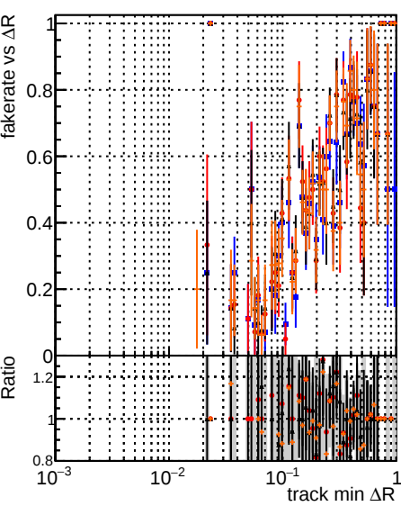
Fake rate vs \Delta R(\text{track, jet}) DOM original, step2, ttbar-phase1-newgeom pixelCPE, template-cut, chiSquare5, step2, ttbar-phase1-newgeom pixelCPE-template-cut-chiSquare5 test
