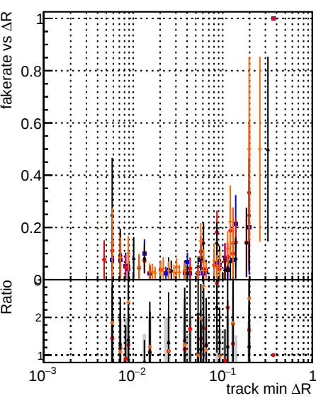
Fake rate vs \Delta R(\text{track}, \text{jet}) DOM original_step2_ttbar_phase1_newgeom DOM pixelCPE template_cut_chiSquare5_step2_ttbar_phase1_newgeom DOM pixelCPE template_cut_chiSquare5_step2_ttbar_phase1_newgeom test
