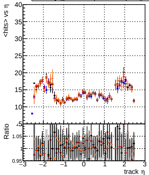
mean hits vs \eta DQM_original_step2_ttbbar-phase1-newgeom DQM_pixelCPETemplate_step2_ttbbar-phase1-newgeom DQM_pixelCPETemplateCutChiSquare15_step2_ttbbar-phase1-newgeom DQM_pixelCPETemplateCutChiSquare5_step2_ttbbar-phase1-newgeom_test
