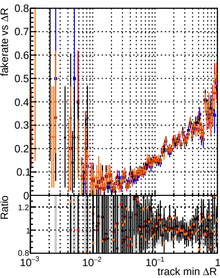
Fake rate vs \Delta R (track, jet) Legend: DOM original_step2_ttbar-phase1-newgeom DOM pixelCPE-template_step2_ttbar-phase1-newgeom DOM pixelCPE-template_chiSquare5_step2_ttbar-phase1-newgeom DOM pixelCPE-template_chiSquare5_step2_ttbar-phase1-newgeom_test
