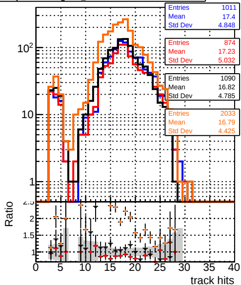
mean hits DQM_original_step2_ttbar-phase1-newgeom DQM_pixelCPETemplate_step2_ttbar-phase1-newgeom DQM_pixelCPETemplateCutChiSquare15_step2_ttbar-phase1-newgeom DQM_pixelCPETemplateCutChiSquare5_step2_ttbar-phase1-newgeom_test
