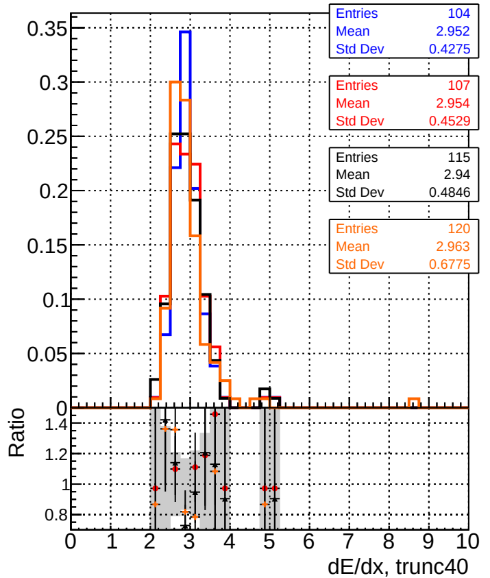
— DQM_original_step2_ttbar-phase1-newgeom — DQM_pixelCPETemplate_step2_ttbar-phase1-newgeom — DQM_pixelCPETemplateCutChiSquare15_step2_ttbar-phase1-newgeom — DQM_pixelCPETemplateCutChiSquare5_step2_ttbar-phase1-newgeom_test
