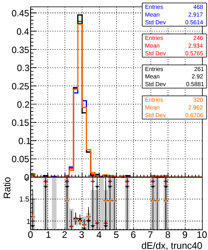
— DQM_original_step2_ttbar-phase1-newgeom — DQM_pixelCPETemplate_step2_ttbar-phase1-newgeom — DQM_pixelCPETemplateCutChiSquare15_step2_ttbar-phase1-newgeom — DQM_pixelCPETemplateCutChiSquare5_step2_ttbar-phase1-newgeom_test
