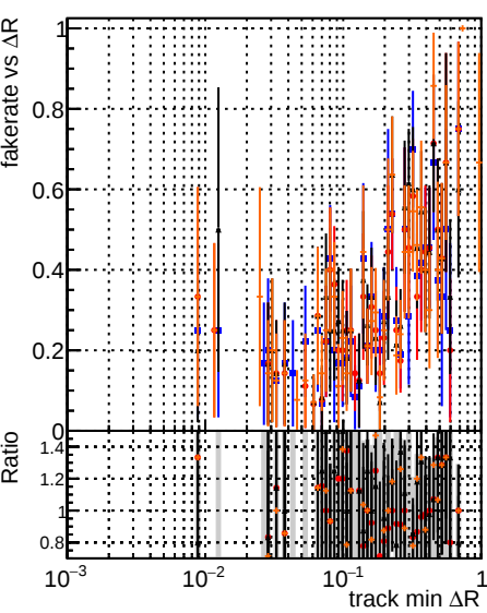
Fake rate vs \Delta R(\text{track, jet}) DOM original step2 ttbar phase1-newgeom DOM pixel CP template step2 ttbar phase1-newgeom DOM pixel CP template cut chi square 5 step2 ttbar phase1-newgeom DOM pixel CP template cut chi square 5 test
