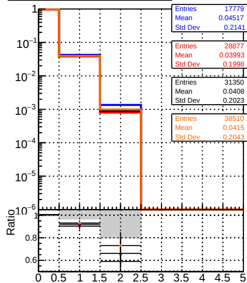
mean hits — DQM_original_step2_ttbar-phase1-newgeom — DQM_pixelCPETemplate_step2_ttbar-phase1-newgeom — DQM_pixelCPETemplateCutChiSquare15_step2_ttbar-phase1-newgeom — DQM_pixelCPETemplateCutChiSquare5_step2_ttbar-phase1-newgeom_test
