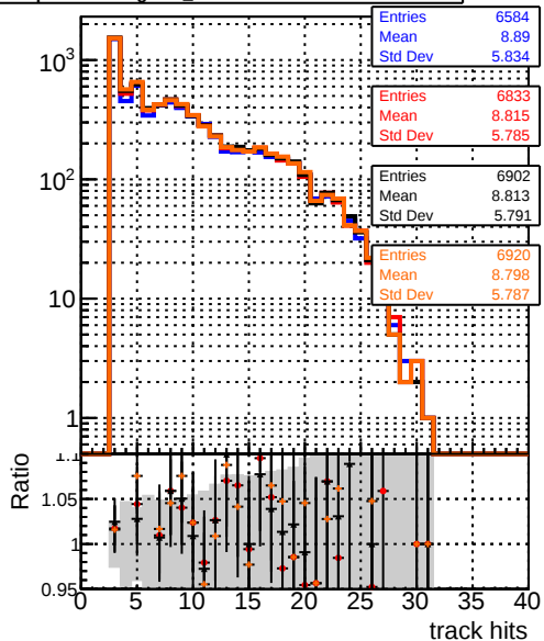
mean hit — DQM_original_step2_ttbar-phase1-newgeom — DQM_pixelCPETemplate_step2_ttbar-phase1-newgeom — DQM_pixelCPETemplateCutChiSquare15_step2_ttbar-phase1-newgeom — DQM_pixelCPETemplateCutChiSquare5_step2_ttbar-phase1-newgeom_test
