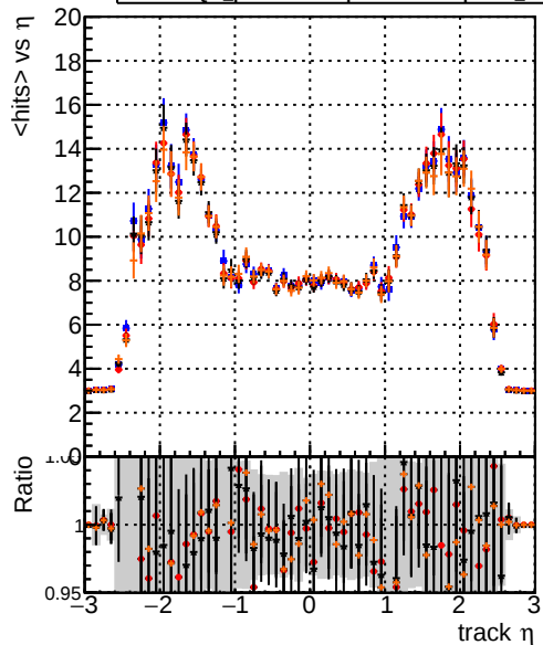
mean hit — DQM_original_step2_ttbar-phase1-newgeom — DQM_pixelCPETemplate_step2_ttbar-phase1-newgeom — DQM_pixelCPETemplateCutChiSquare15_step2_ttbar-phase1-newgeom — DQM_pixelCPETemplateCutChiSquare5_step2_ttbar-phase1-newgeom_test
