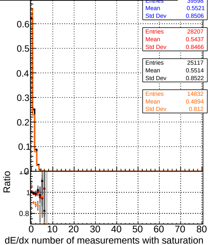
—■— DQM_original_step2_ttbbar-phase1-newgeom —●— DQM_pixelCPETemplate_step2_ttbbar-phase1-newgeom —■— DQM_pixelCPETemplateCutChiSquare15_step2_ttbbar-phase1-newgeom —■— DQM_pixelCPETemplateCutChiSquare5_step2_ttbbar-phase1-newgeom_test
