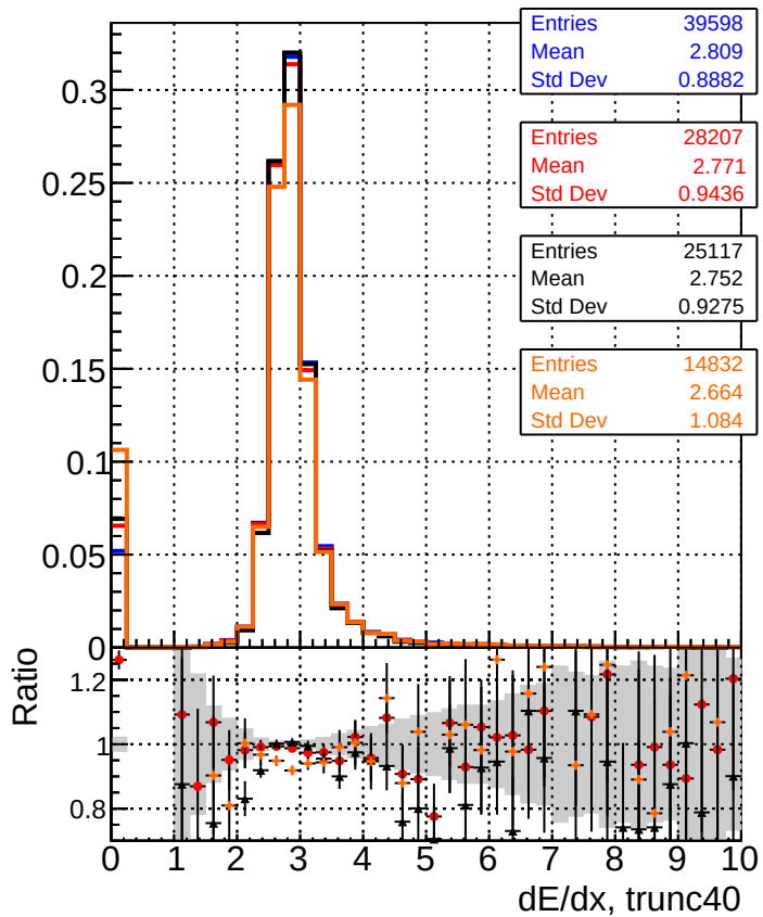
—■— DQM_original_step2_ttbbar-phase1-newgeom —●— DQM_pixelCPETemplate_step2_ttbbar-phase1-newgeom —■— DQM_pixelCPETemplateCutChiSquare15_step2_ttbbar-phase1-newgeom —■— DQM_pixelCPETemplateCutChiSquare5_step2_ttbbar-phase1-newgeom_test
