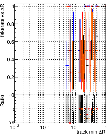
Fake rate vs \Delta R(\text{track, jet}) DQM original_step2_ttbarm-phase1-newgeom DQM pixelCPE-template_step2_ttbarm-phase1-newgeom DQM pixelCPE-template_ChiSquare5_step2_ttbarm-phase1-newgeom DQM pixelCPE-template_ChiSquare5_step2_ttbarm-phase1-newgeom test
