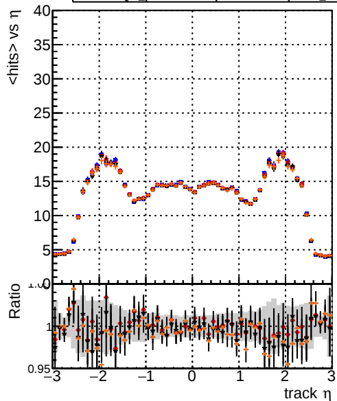
mean hit DQM_original_step2_ttbar-phase1-newgeom DQM_pixelCPETemplate_step2_ttbar-phase1-newgeom DQM_pixelCPETemplateCutChiSquare15_step2_ttbar-phase1-newgeom DQM_pixelCPETemplateCutChiSquare5_step2_ttbar-phase1-newgeom_test
