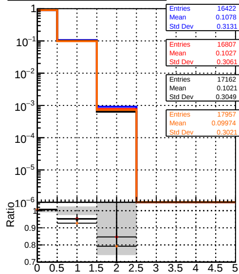
mean hit DQM_original_step2_ttbar-phase1-newgeom DQM_pixelCPETemplate_step2_ttbar-phase1-newgeom DQM_pixelCPETemplateCutChiSquare15_step2_ttbar-phase1-newgeom DQM_pixelCPETemplateCutChiSquare5_step2_ttbar-phase1-newgeom_test
