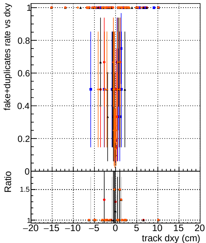
DQM_original_step2_ttbar-phase1-newgeom DQM_pixelCPETemplate_step2_ttbar-phase1-newgeom DQM_pixelCPETemplateCutChiSquare15_step2_ttbar-phase1-newgeom DQM_pixelCPETemplateCutChiSquare5_step2_ttbar-phase1-newgeom_test
