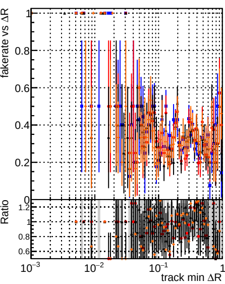
Fake rate vs \Delta R(\text{track, jet}) DOM original_step2_ttbbar-phase1-newgeom DOM pixel_CDF-template_step2_ttbbar-phase1-newgeom DOM pixel_CDF-templateCut_ChiSquare5_step2_ttbbar-phase1-newgeom DOM pixel_CDF-templateCut_ChiSquare5_step2_ttbbar-phase1-newgeom_test
