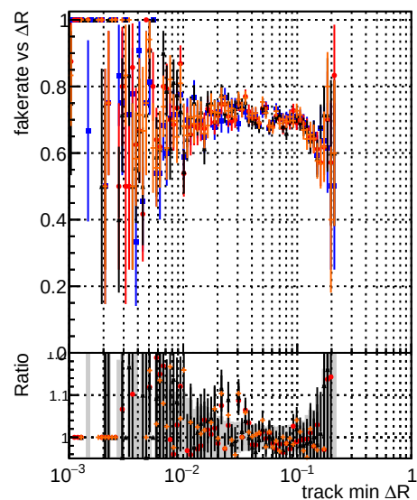
DOM original step2 ttbar phase1-newgeom DOM pixel CDF template step2 ttbar phase1-newgeom DOM pixel CDF template cut chiSquare5 step2 ttbar phase1-newgeom DOM pixel CDF template cut chiSquare5 step2 ttbar phase1-newgeom test
