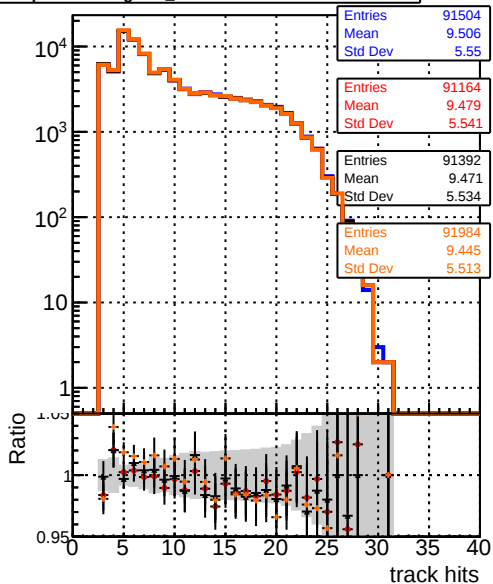
mean hits Legend: Blue line: DQM_original_step2_ttbar-phase1-newgeom Red line with dots: DQM_pixelCPETemplate_step2_ttbar-phase1-newgeom Black line with dots: DQM_pixelCPETemplateCutChiSquare15_step2_ttbar-phase1-newgeom Orange line with dots: DQM_pixelCPETemplateCutChiSquare5_step2_ttbar-phase1-newgeom_test
