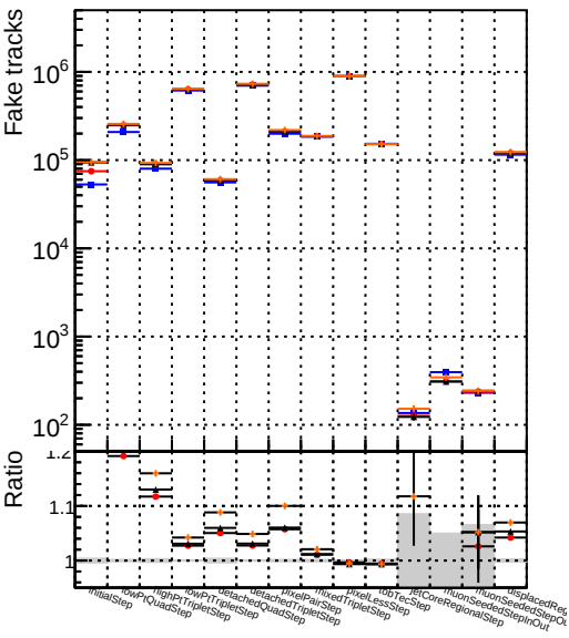
Number Legend Model 1 DQM pixelCPETemplateCutChiSquare15_step2_ttbbar-phase1-newgeom 2 DQM pixelCPETemplateCutChiSquare15_step2_ttbbar-phase1-newgeom_test 3 DQM pixelCPETemplateCutChiSquare15_step2_ttbbar-phase1-newgeom 4 DQM pixelCPETemplateCutChiSquare5_step2_ttbbar-phase1-newgeom_test
