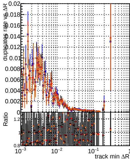
—•— DOM original_step2_ttbare-phase1-newgeom —•— DOM pixelCPE-template_step2_ttbare-phase1-newgeom —•— DOM pixelCPE-template_chiSquare5_step2_ttbare-phase1-newgeom —•— DOM pixelCPE-template_chiSquare5_step2_ttbare-phase1-newgeom_test
