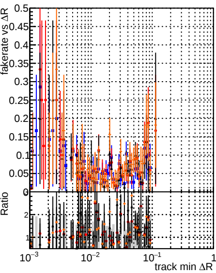
Fake rate vs \Delta R(\text{track}, \text{jet}) Legend: DOM original_step2_ttbbar-phase1-newgeom DOM pixelCPE-template_step2_ttbbar-phase1-newgeom DOM pixelCPE-template-cut-chisquare5_step2_ttbbar-phase1-newgeom DOM pixelCPE-template-cut-chisquare5_step2_ttbbar-phase1-newgeom_test
