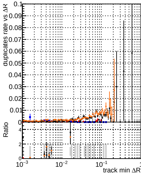
DOM original_step2_ttbar-phase1-newgeom DOM pixelCDETemplate_step2_ttbar-phase1-newgeom DOM pixelCDETemplate_ChiSquare5_step2_ttbar-phase1-newgeom DOM pixelCDETemplate_ChiSquare5_step2_ttbar-phase1-newgeom_test
