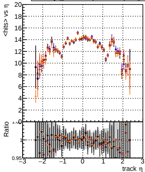
mean hits DQM_original_step2_ttbbar-phase1-newgeom DQM_pixelCPETemplate_step2_ttbbar-phase1-newgeom DQM_pixelCPETemplateCutChiSquare15_step2_ttbbar-phase1-newgeom DQM_pixelCPETemplateCutChiSquare5_step2_ttbbar-phase1-newgeom_test
