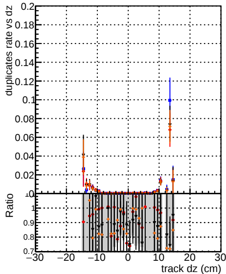
Square15 step2 ttbar-ph Square5 step2 ttbar-ph
