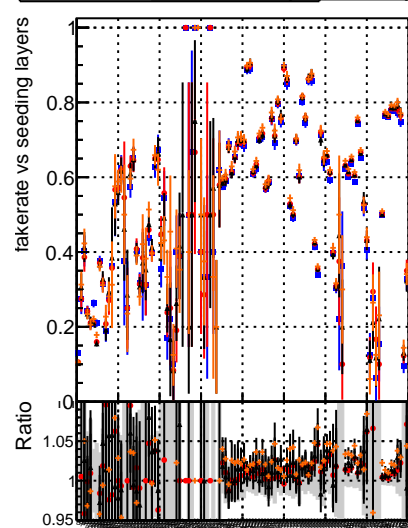
Fake rate vs. — DCM-original-step2-tbar-phase1-newgeom — DCM-pixelCPE-template-step2-tbar-phase1-newgeom — DCM-pixelCPE-template-curves-step2-tbar-phase1-newgeom — DCM-pixelCPE-template-curves-squares-step2-tbar-phase1-newgeom-test
