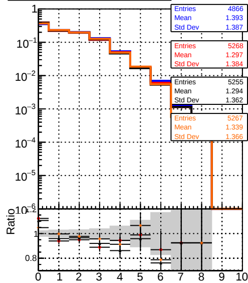
mean hits — DQM_original_step2_ttbar-phase1-newgeom — DQM_pixelCPETemplate_step2_ttbar-phase1-newgeom — DQM_pixelCPETemplateCutChiSquare15_step2_ttbar-phase1-newgeom — DQM_pixelCPETemplateCutChiSquare5_step2_ttbar-phase1-newgeom_test
