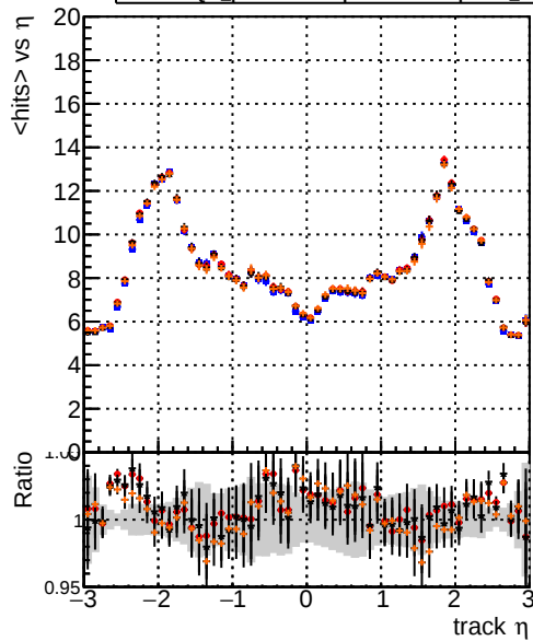
mean hits vs \eta DQM_original_step2_ttbar-phase1-newgeom DQM_pixelCPETemplate_step2_ttbar-phase1-newgeom DQM_pixelCPETemplateCutChiSquare15_step2_ttbar-phase1-newgeom DQM_pixelCPETemplateCutChiSquare5_step2_ttbar-phase1-newgeom_test
