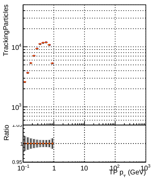
—●— DQM_original_step2_ttbar-phase1-newgeom —●— DQM_pixelCPETemplate_step2_ttbar-phase1-newgeom —●— DQM_pixelCPETemplateCutChiSquare5_step2_ttbar-phase1-newgeom —●— DQM_pixelCPETemplateCutChiSquare5_step2_ttbar-phase1-newgeom_test
