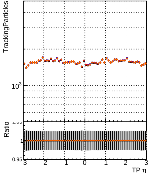
—●— DQM_original_step2_ttbar-phase1-newgeom —●— DQM_pixelCPETemplate_step2_ttbar-phase1-newgeom —●— DQM_pixelCPETemplateCutChiSquare5_step2_ttbar-phase1-newgeom —●— DQM_pixelCPETemplateCutChiSquare5_step2_ttbar-phase1-newgeom_test
