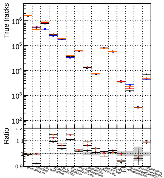
Number of tracks vs collection Legend: DQM_original_step2_ttbar-phase1-newgeom DQM_pixelCPETemplate_step2_ttbar-phase1-newgeom DQM_pixelCPETemplateCutChiSquare5_step2_ttbar-phase1-newgeom DQM_pixelCPETemplateCutChiSquare5_step2_ttbar-phase1-newgeom_test
