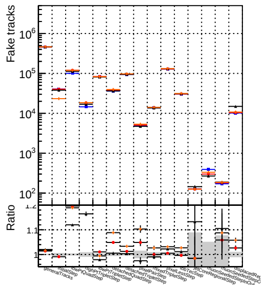
Number of tracks vs collection DQM_original_step2_ttbar-phase1-newgeom DQM_pixelCPETemplate_step2_ttbar-phase1-newgeom DQM_pixelCPETemplateCutChiSquare5_step2_ttbar-phase1-newgeom DQM_pixelCPETemplateCutChiSquare5_step2_ttbar-phase1-newgeom_test
