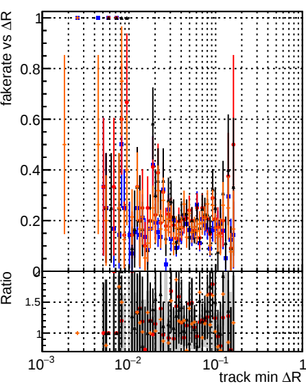
Fake rate vs \Delta R(\text{track, jet}) DOM original step2 ttbar phase1-newgeom DOM pixelCDE template step2 ttbar phase1-newgeom DOM pixelCDE chi-squares step2 ttbar phase1-newgeom DOM pixelCDE template cut chi-squares step2 ttbar phase1-newgeom test
