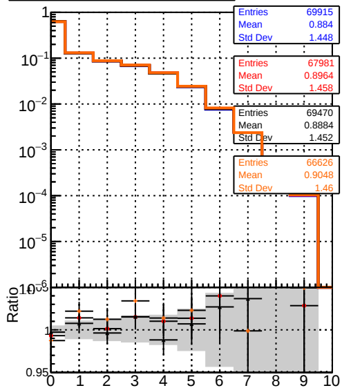
— DQM_original_step2_ttbar-phase1-newgeom — DQM_pixelCPETemplate_step2_ttbar-phase1-newgeom — DQM_pixelCPETemplateCutChiSquare5_step2_ttbar-phase1-newgeom — DQM_pixelCPETemplateCutChiSquare5_step2_ttbar-phase1-newgeom_test
